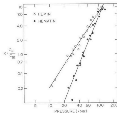
FIG. 4. \ln K vs \ln P —Crystals with weak coupling between sites.
